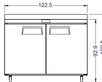
MGF8413-MFR48"
